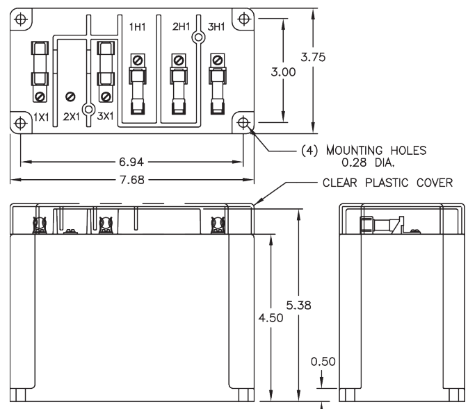
Model EI-2VT460-480FF
