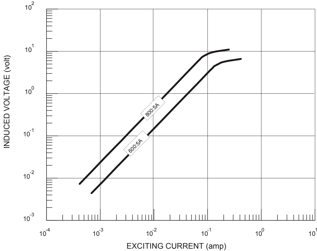
TYPICAL EXCITATION CURVE for MODEL 3SP at 60HZ
