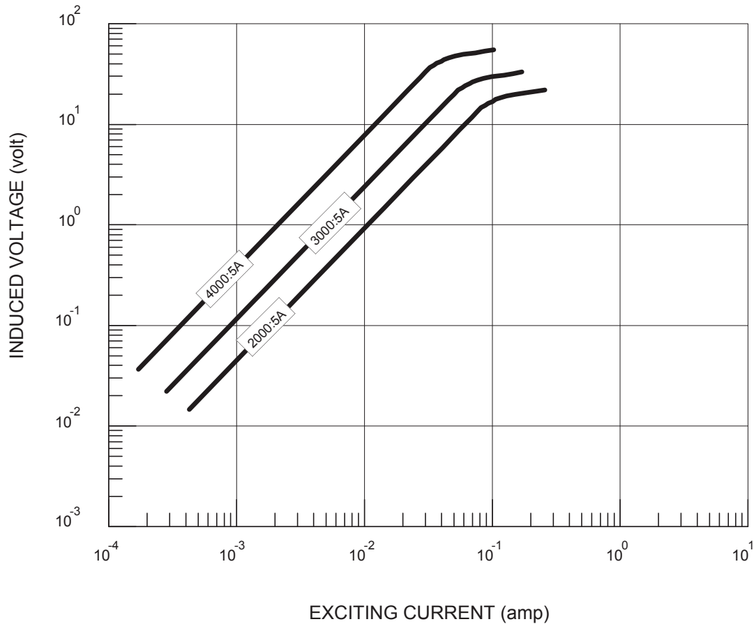
TYPICAL EXCITATION CURVE for MODEL 91SP at 60HZ
