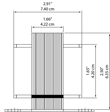
Side Dimensions
